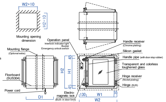
BHPB06-□□□R (Electromagnetic lock)
