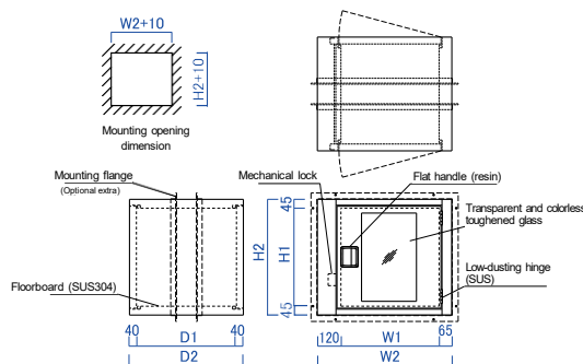
EPB06-□□□R (Mechanical lock)
