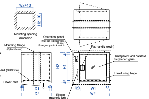
BHPB06-□□□R (Electromagnetic lock)
